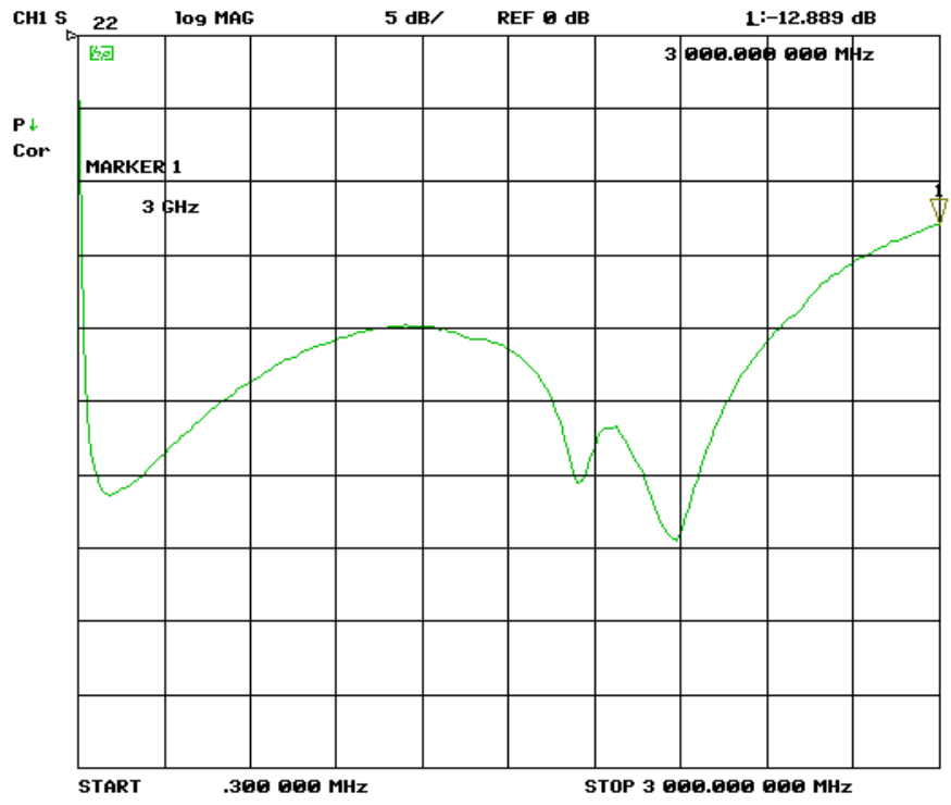
Picture 16 – TBWA2/20dB, output return loss, IS22, 300 kHz – 3 GHz, lin.
