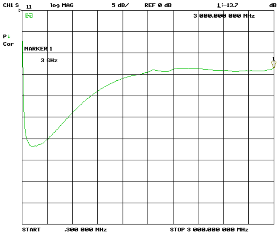
Picture 15 – TBWA2/20dB, input return loss, IS11, 300 kHz – 3 GHz, lin.
