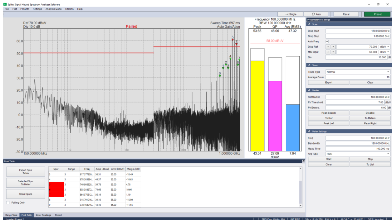
Figure 25 : Radiated Emissions Precompliance Testing for the VSG25A
