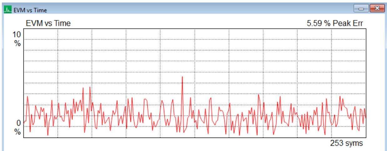
Figure 24 : EVM vs Time plot
