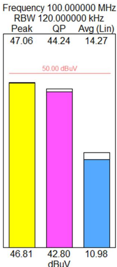
Figure 29: Bar Meters Measuring Pulsed Signal
