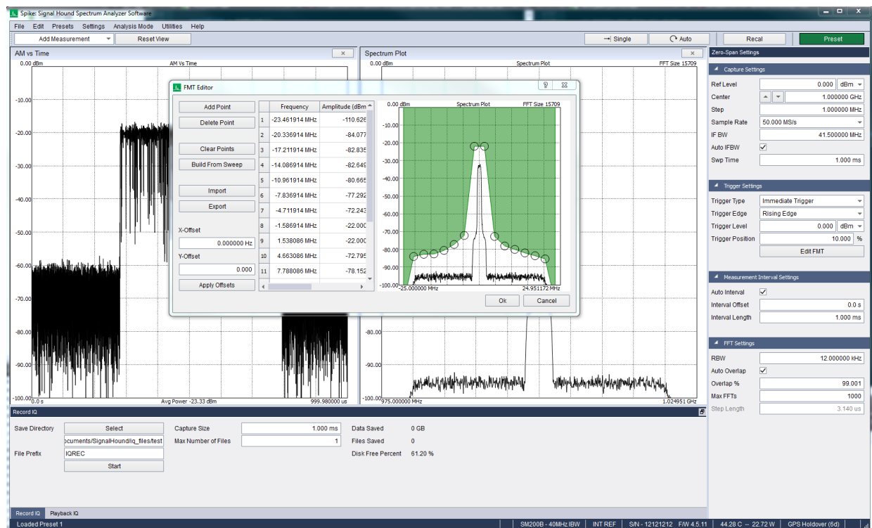
Figure 5: FMT editor
